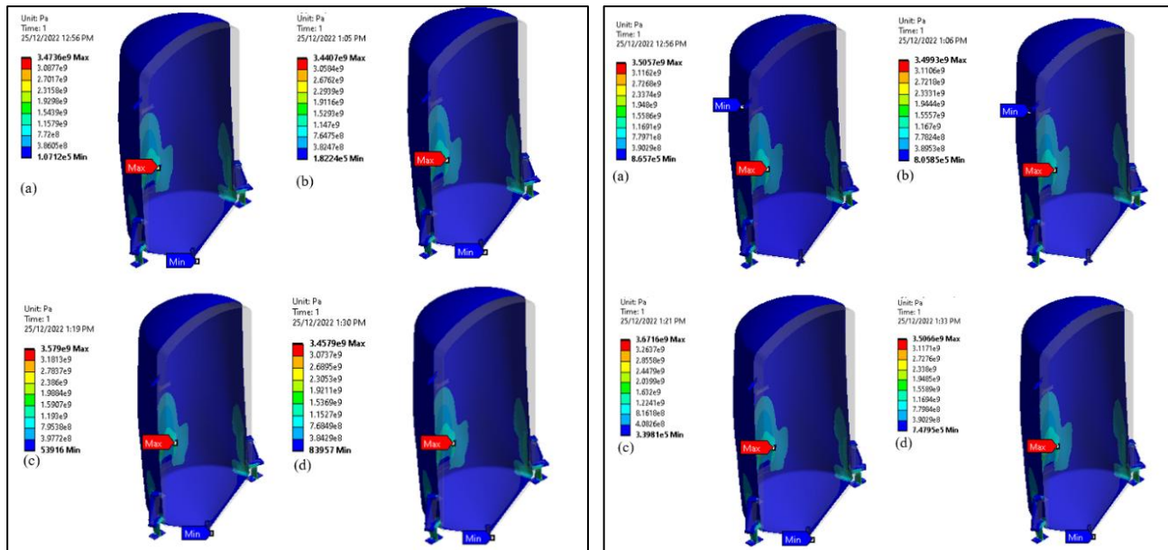
Fig. 6. 35°C initial temperature (a) Stainless steel (b) Carbon steel (c) Titanium alloy (d) Super duplex 2507
