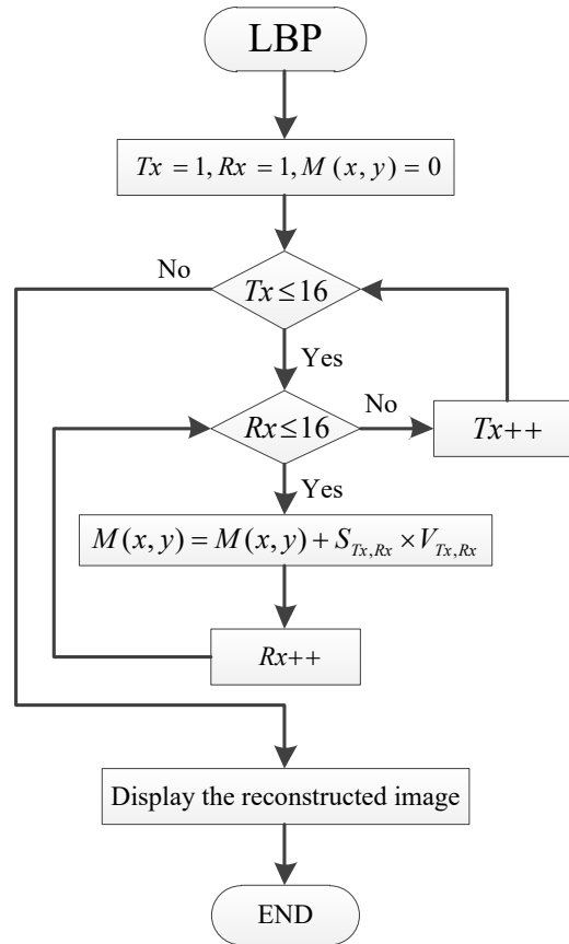
Fig. 1. LBP algorithm flowchart
