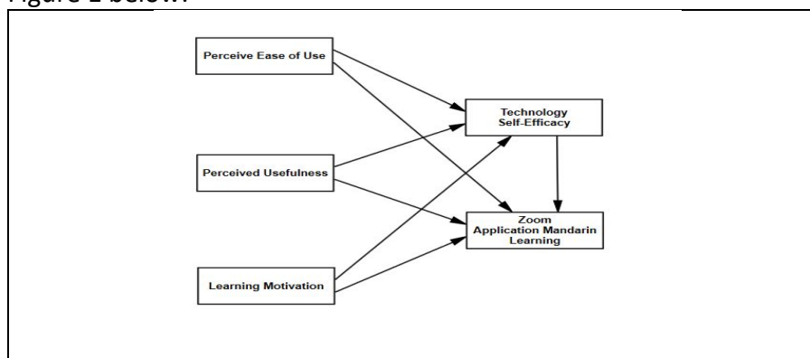
Fig. 1. Theoretical framework
