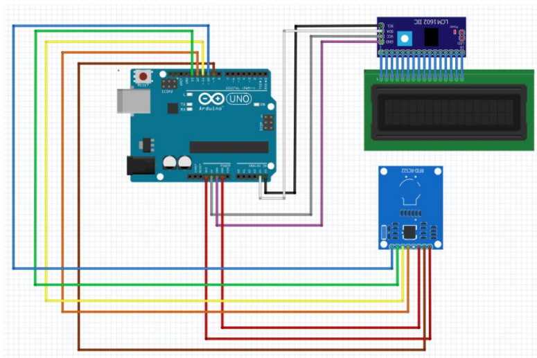
Fig. 2. Circuit diagram
