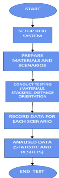
Fig. 1. Research flowchart
