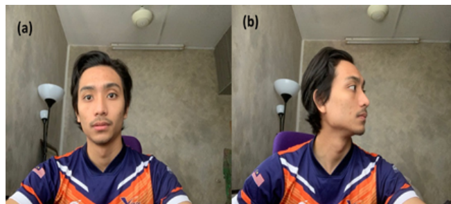
Fig. 1. Pose variation
