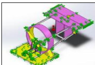
Fig. 5. Fixtures for horizontal tail
