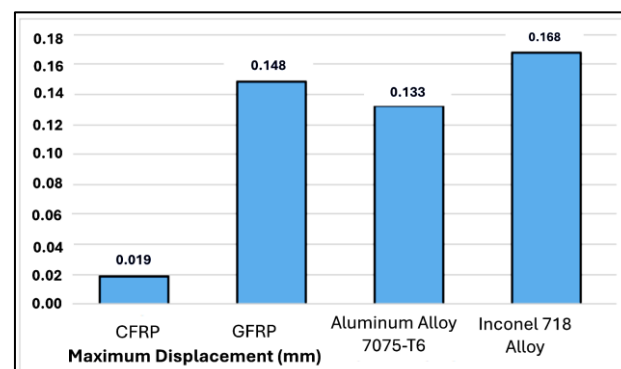
Fig. 26. Results of maximum displacement for all materials on horizontal tail
