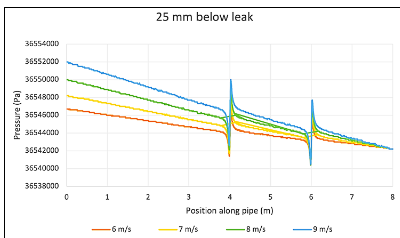
Fig. 20. Pressure behavior around the leaks between different fluid Velocity along the pipe at 25 mm below the leaks
