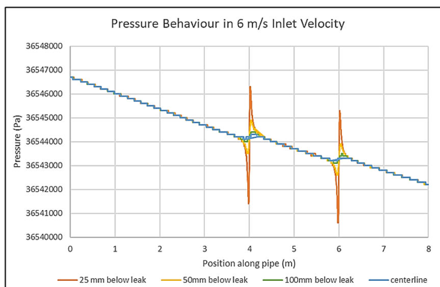
Fig. 8. Pressure distribution along pipeline for different positions at 6\text{ m/s}
