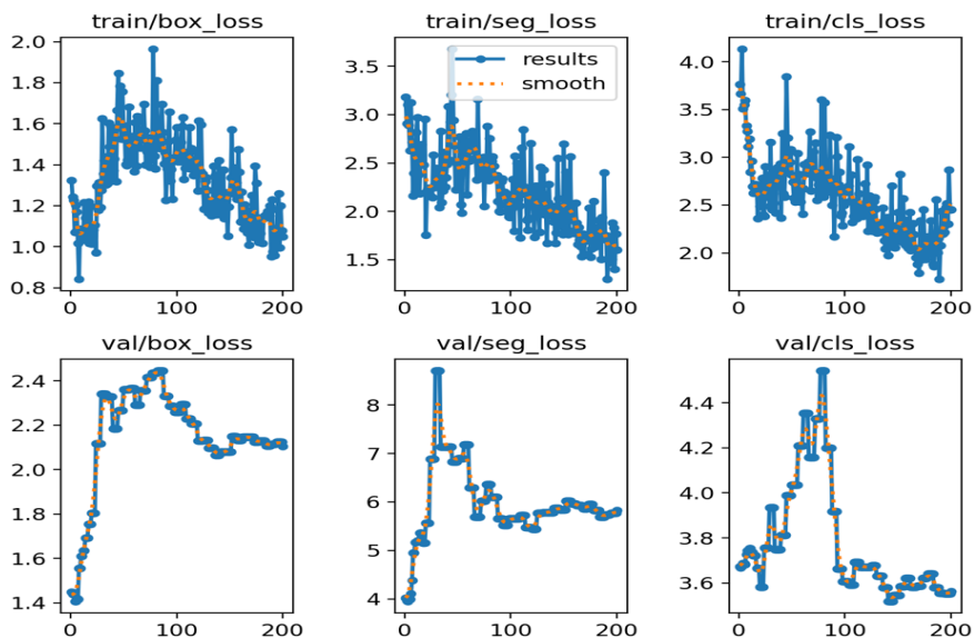
Fig. 7. Loss rate curves
