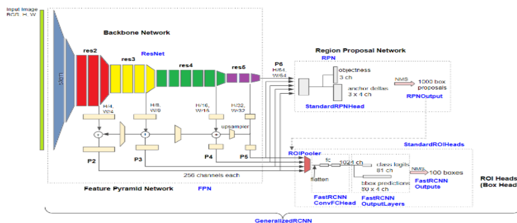
Fig. 2. Architecture of Detectron2
