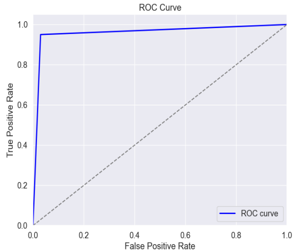
Fig. 9. ROC curve
