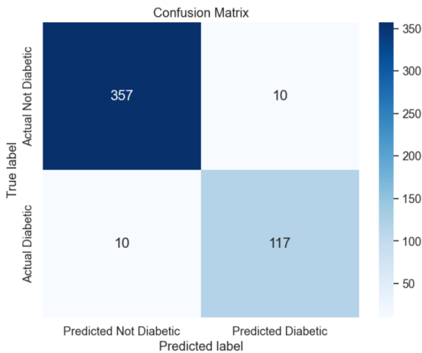
Fig. 8. Confusion matrix
