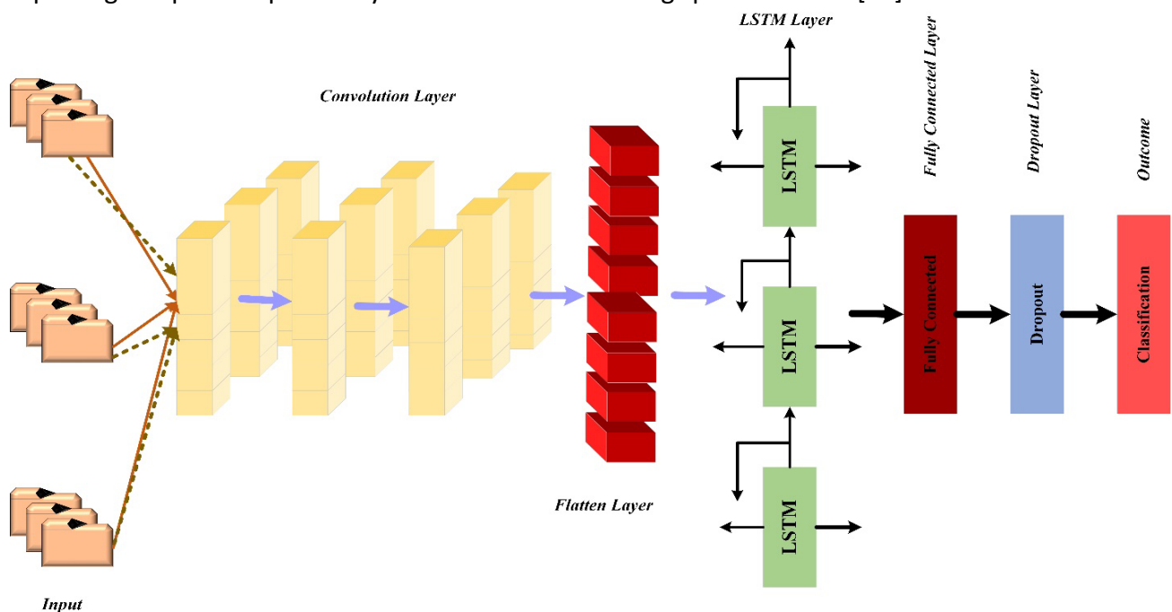
Fig. 2. Architecture of hybrid CNN-LSTM
