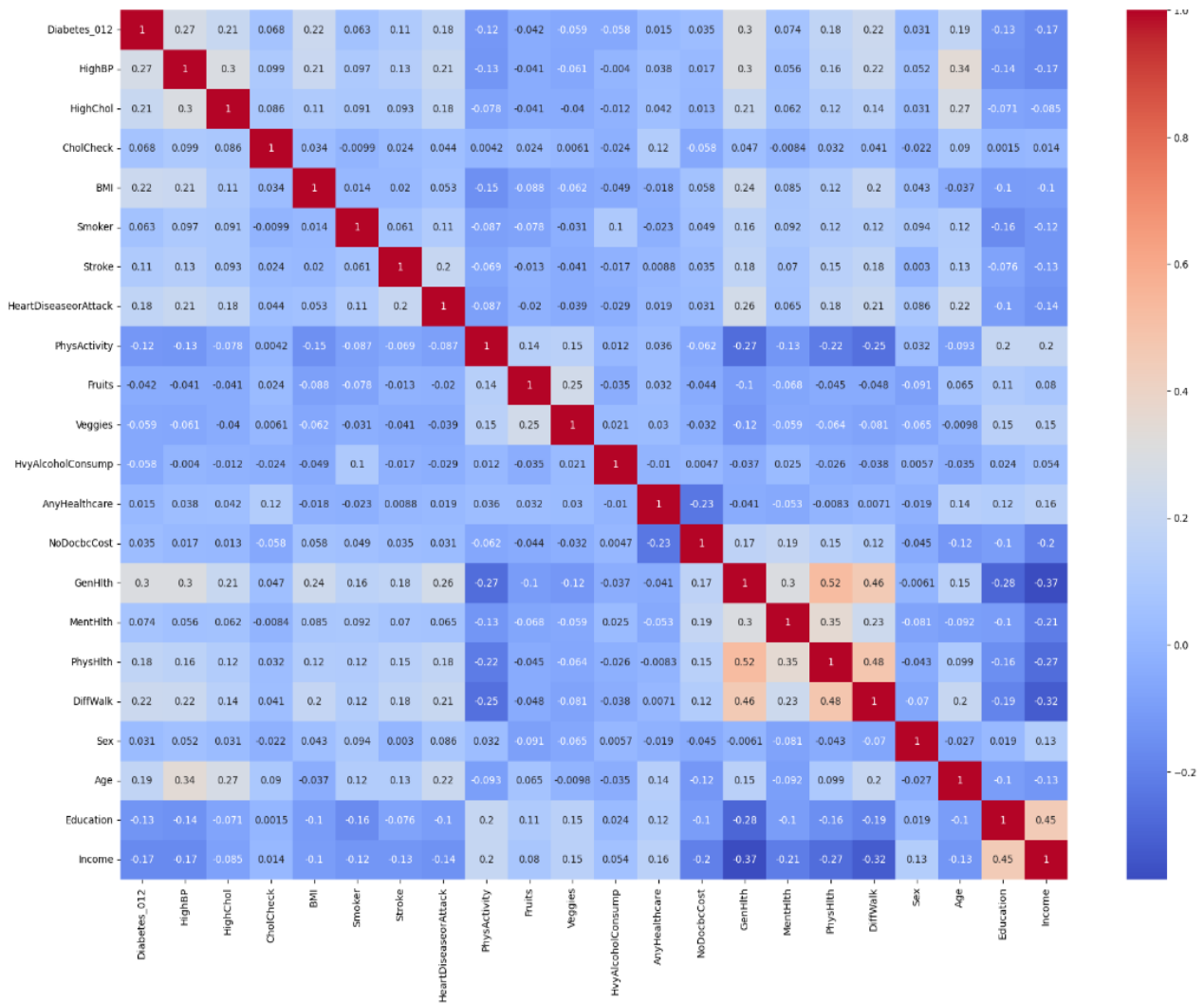
Fig. 6. Correlation matrix
