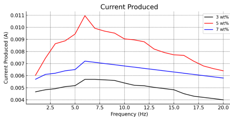
Fig. 4. Effect of different weight percent and frequency on current produced
