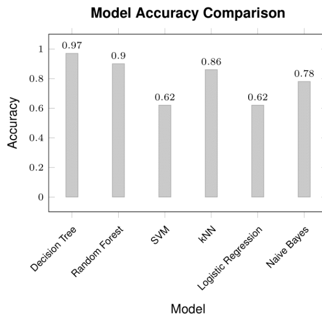
Fig. 7. Accuracy performance for each of the model
